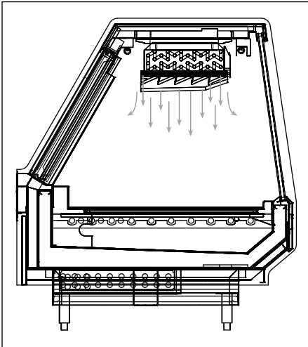
Fig. 12 Airflow pattern
