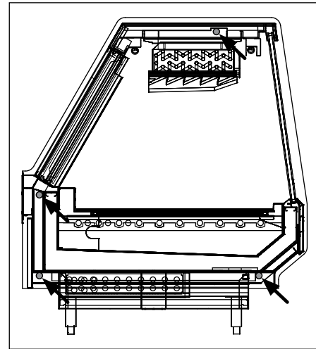
Fig. 3 Bolt locations
